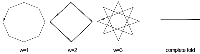
Figure 2. Regular stars for n = 8 with positive winding numbers.
