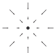
\text{ind}=+1
