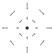
\text{ind}=-1
